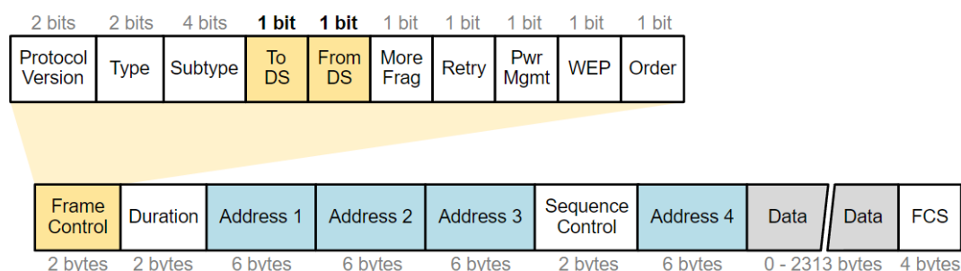
Figure 5. 802.11 Frame Format.
