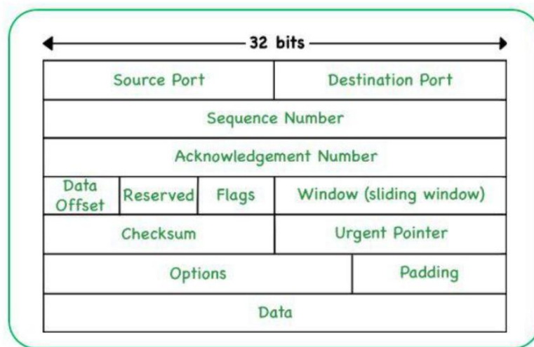
Diagram Showing the TCP packet Format
