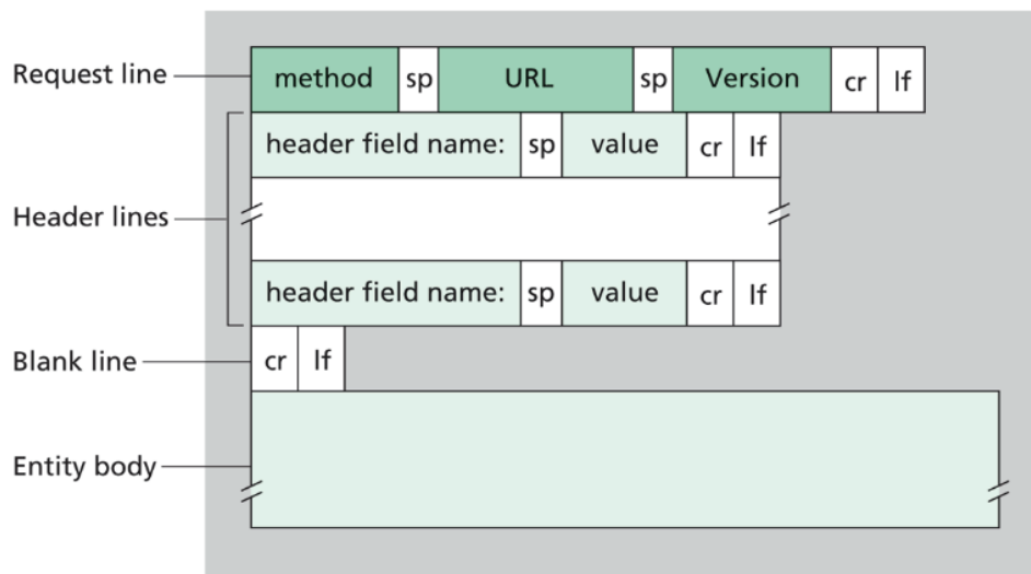
Figure 2.8 ♦ General format of a request message
